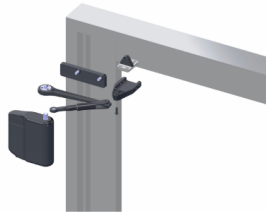
ADA EZ PRO Operator Non-Handed Push Side Mounting - Parallel Arm Black Cover - Standard
